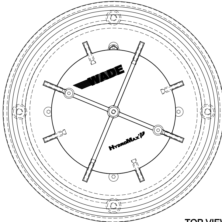
TOP VIEW ( DOME REMOVED)
