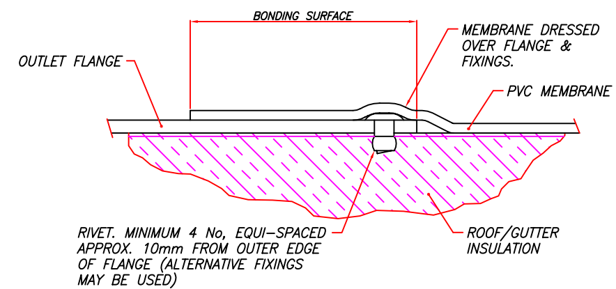
OUTLET FIXING DETAIL
