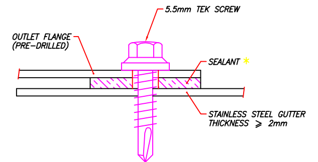
OUTLET FIXING DETAIL SCALE 1:1
