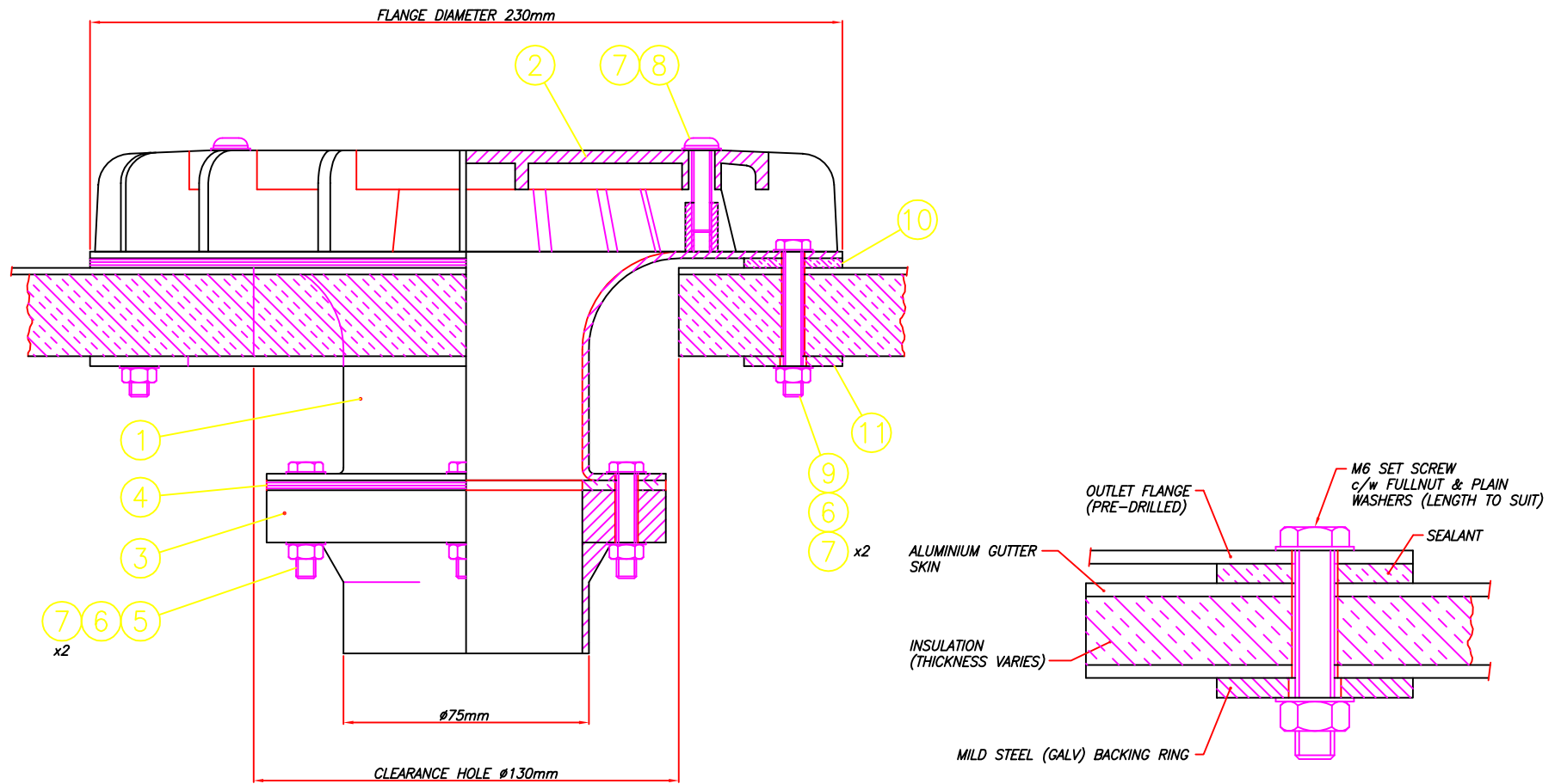
OUTLET FIXING DETAIL SCALE 1:1
