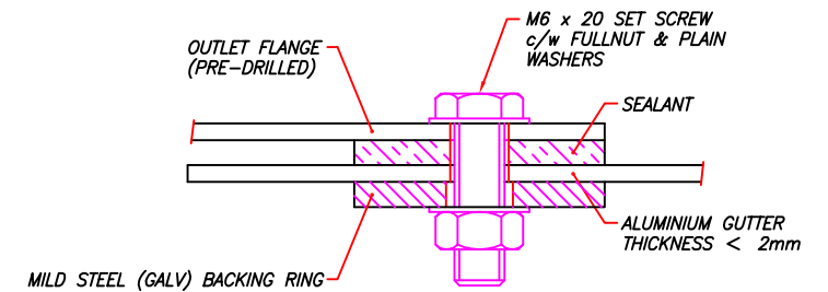
OUTLET FIXING DETAIL SCALE 1:1
