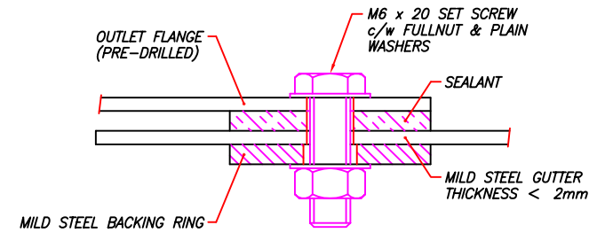
OUTLET FIXING DETAIL SCALE 1:1
