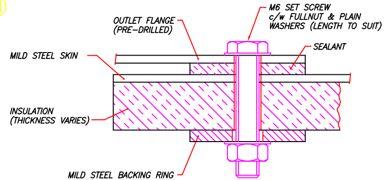
OUTLET FIXING DETAIL SCALE 1:1
