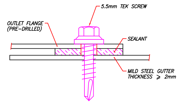
OUTLET FIXING DETAIL SCALE 1:1
