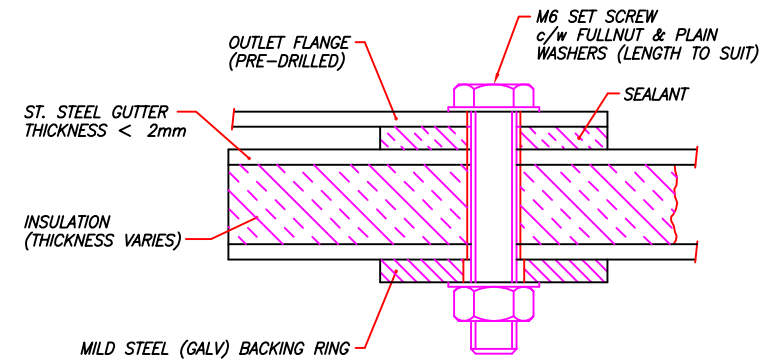
OUTLET FIXING DETAIL
