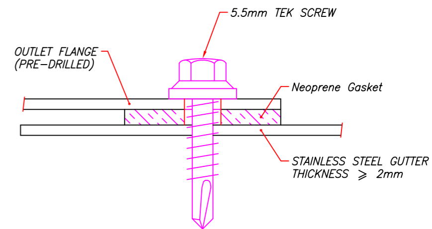
OUTLET FIXING DETAIL SCALE 1:1
